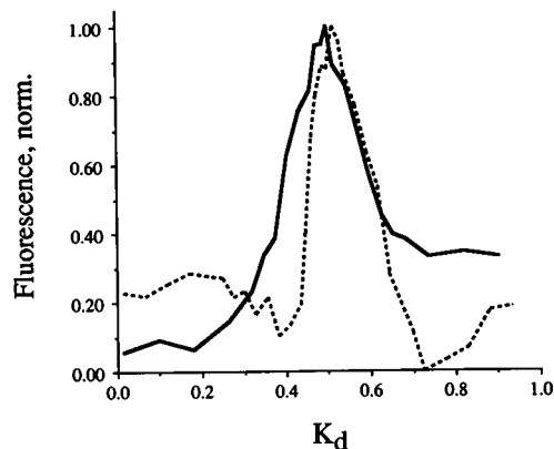
FIGURE 1 Sepharose CL-6B gel filtration of Triton X-100 (solid line) and reduced Triton X-100 (dotted line) with both peaks normalized to 1.0. V_0 and V_1 were determined by gel filtration of FITC-dextran 2000 and potassium ferricyanide, respectively, and their values were both determined for elution buffer containing Triton X-100 and reduced Triton X-100 (see Methods for a complete description). 0.0 on the x-axis indicates the void volume while 1.0 indicates the total elution volume.
