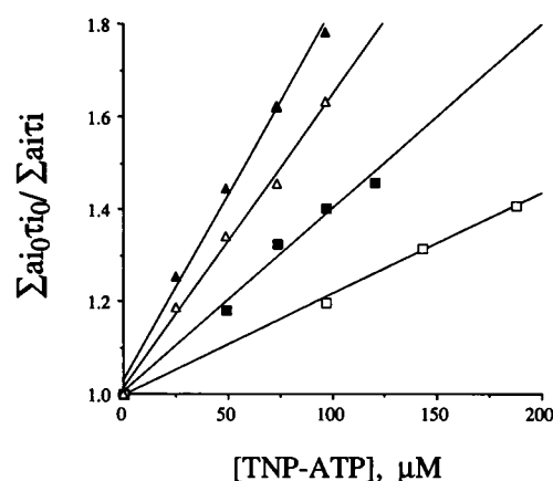
FIGURE 4 Stern-Volmer plots of TNP-ATP quenching of the fluorescence decay of ANT-CAT in reduced Triton X-100 micelles at four different values of \alpha_{pm} . (□) ANT-CAT, 0.214 mg/ml, in 0.934% (wt/vol) reduced Triton X-100, (■) two-fold dilution of the original concentration with buffer containing no detergent, (Δ) four-fold dilution of the original concentration, (▲) eight-fold dilution of the original concentration. The excitation wavelength was 290 nm with emission monitored at 345 nm. TNP-ATP was added to the sample from a 3.0 mM stock and TNP-ATP concentrations shown on the x-axis were adjusted for dilution (see Methods for complete description). The y-axis shows the average decay time of ANT-CAT without TNP-ATP added ( \sum a_i0\tau_i0 ) divided by ANT-CAT the corresponding values with TNP-ATP present, also called the quenching ratio.
