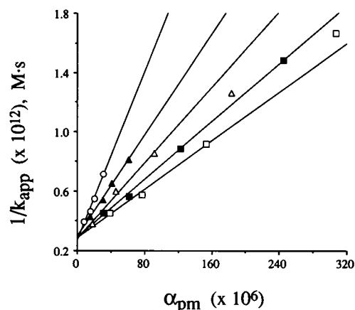
FIGURE 5 Reciprocal apparent quenching constant versus \alpha_{pm} at constant \alpha_m/\alpha_{pm} . (□) \alpha_m/\alpha_{pm} = 29.1 , (■) \alpha_m/\alpha_{pm} = 36.7 , (Δ) \alpha_m/\alpha_{pm} = 49.2 , (▲) \alpha_m/\alpha_{pm} = 74.3 , (○) \alpha_m/\alpha_{pm} = 149.7 . The first set of points (□) were calculated from the slopes shown in Fig. 3. The subsequent sets of points were obtained in the same manner using samples which contained less ANT-CAT and increasing amounts of reduced Triton X-100; however, each set of points has a constant \alpha_m/\alpha_{pm} . The slopes and intercepts from this plot are referred to as S1 and I1, respectively.
